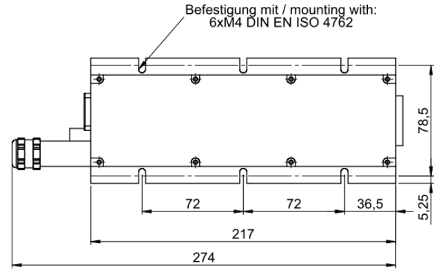
OEM-Controller
